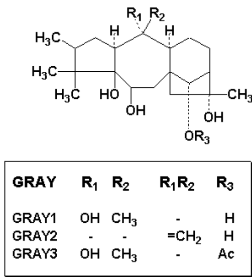
Figure 9. Grayanotoxins [173].
